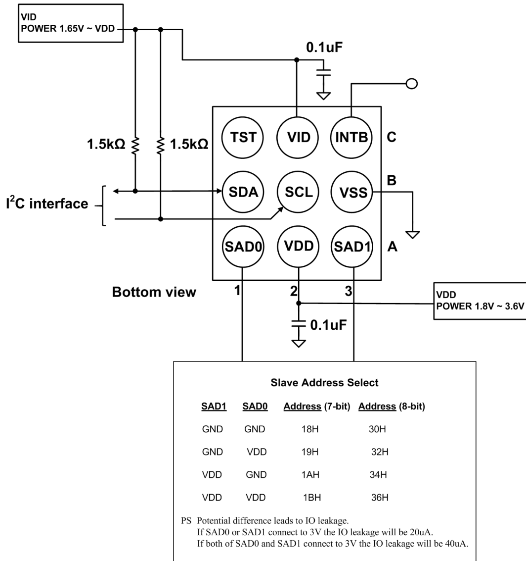
Figure 4. Application Circuit
