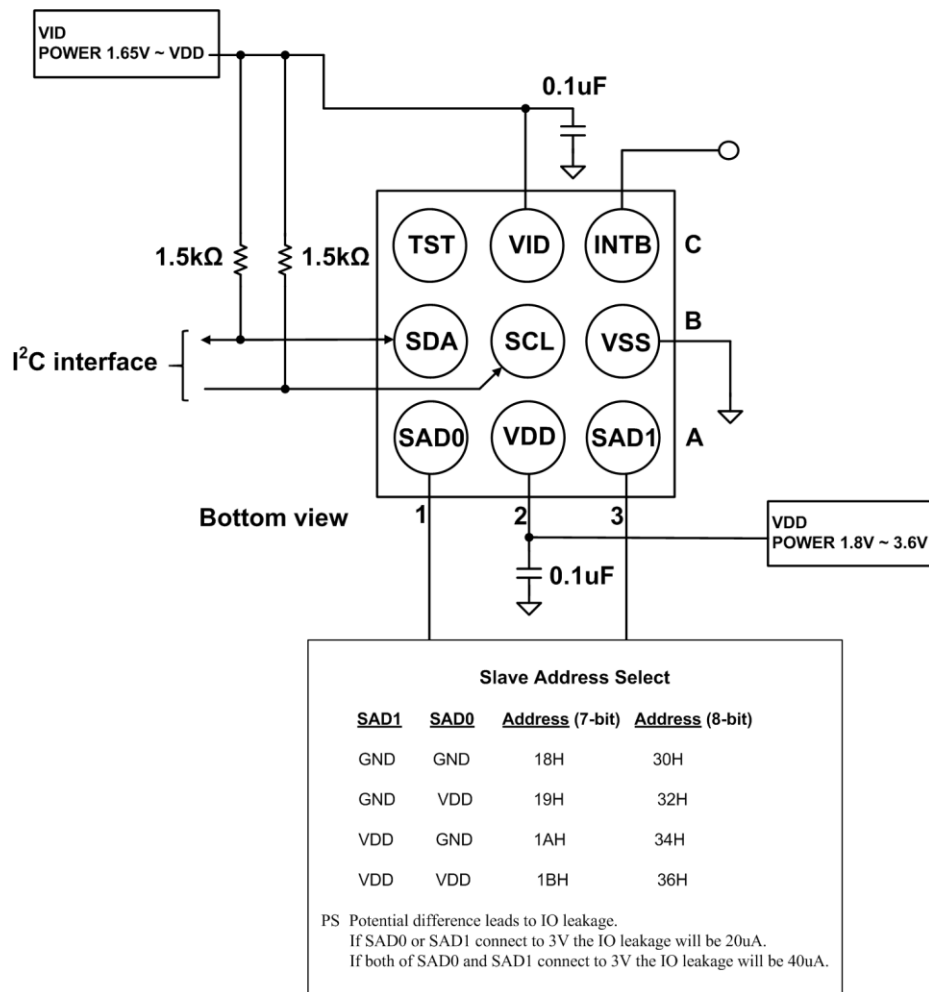
Figure 4. Application Circuit
